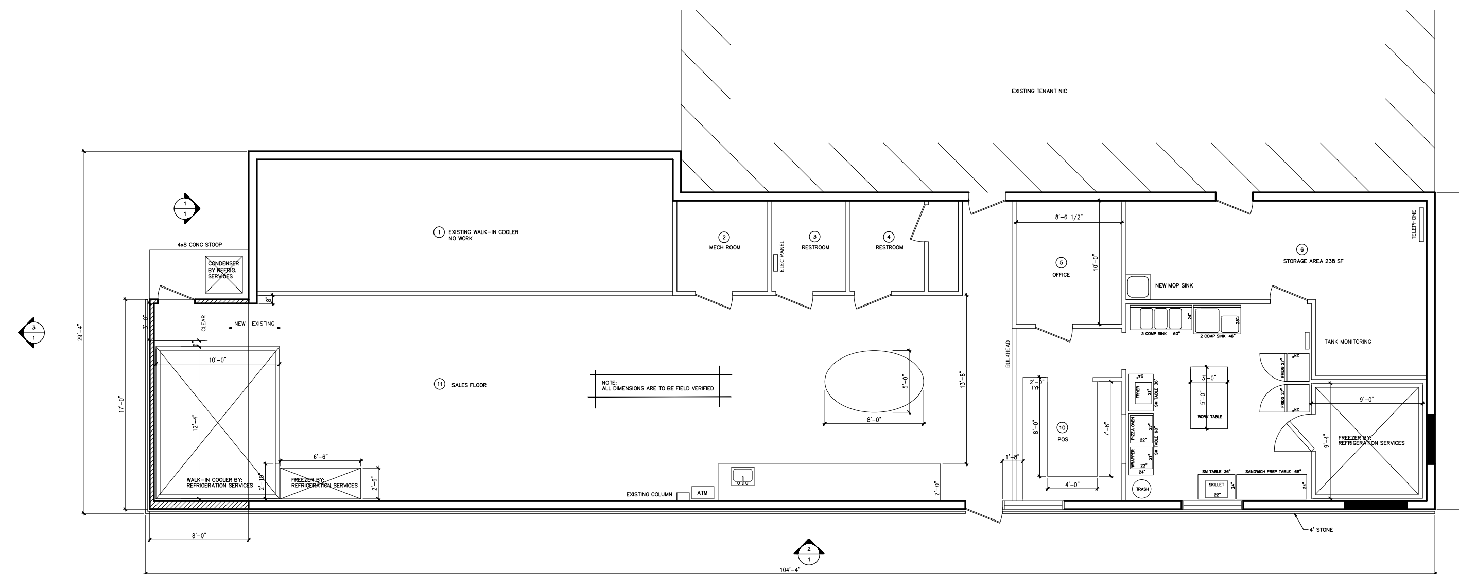
PROPOSED PLAN Scale: 1/4" = 1'-0"
